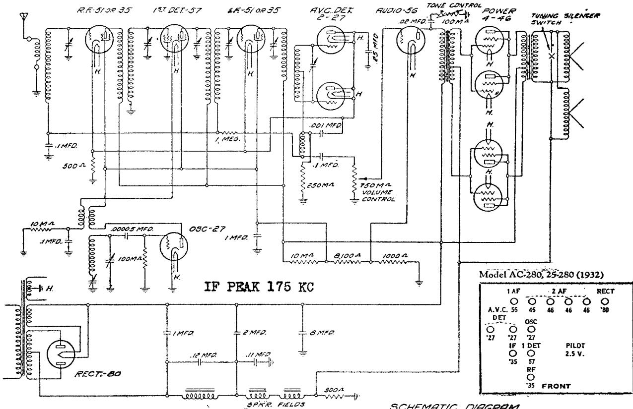
SCHEMATIC DIAGRAM of CLARION MODEL-280 DRAWN BY: J.M. CHECKED: APPROVED: DATE: 6-10-32
